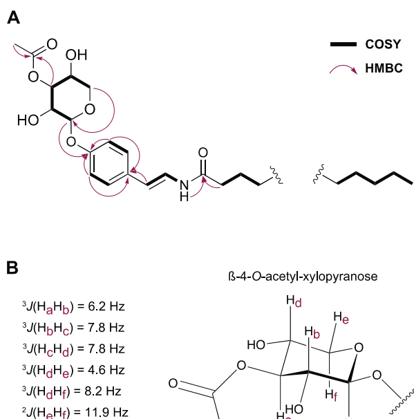
Figure 1. Structure elucidation of hyellamide ( 1 ). (A) Key HMBC and COSY correlations obtained from NMR analysis of 1 . (B) Coupling constant analysis establishing the relative configuration of the acetylated xylose residue in 1 .
