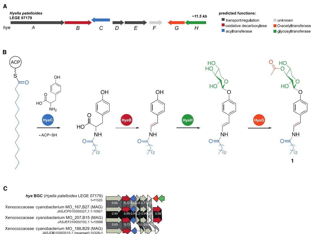
Figure 2. Proposed biosynthesis of hyellamide ( 1 ). (A) Organization of the hye BGC of Hyella patelloides LEGE 07179, proposed to be involved in the biosynthesis of 1 . (B) Proposed biosynthesis steps leading to the production of 1 . (C) Additional hye -like BGCs found in publicly available cyanobacterial genomes/MAGs (minimum of 30% of similarity and 50% of query coverage), homologous genes in different clusters are connected through shaded regions, darker shaded indicate higher identity.
