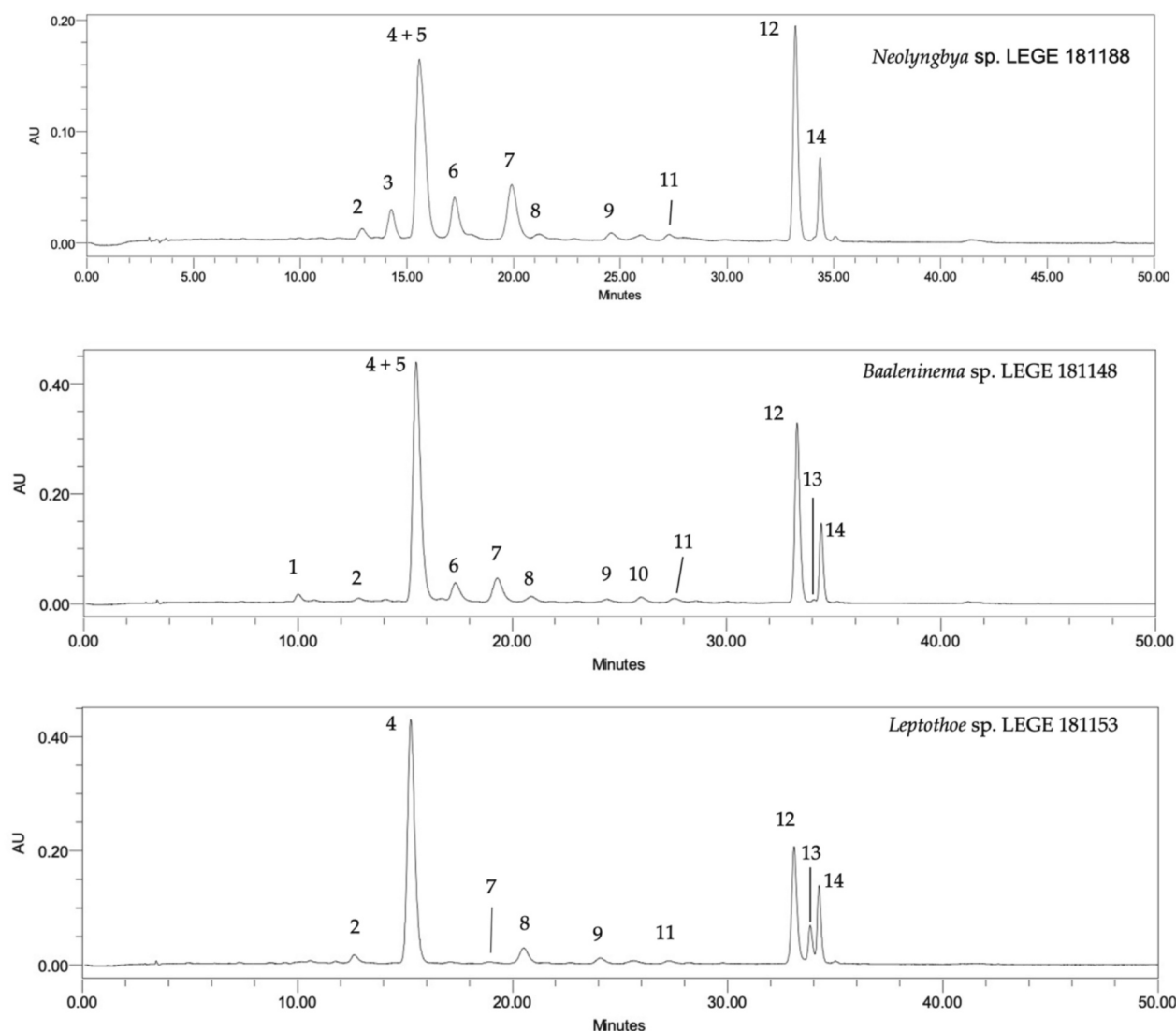
Fig. 3. Carotenoid and chlorophylls profile of acetonic extracts of cyanobacteria strains. HPLC-PDA recorded at 450 nm. Chlorophyll- a derivatives (1 and 6), Lutein (2), \beta -carotene oxygenated derivative (3,8 and 9), Zeaxanthin (4), Chlorophyll- a (5), Myxoxanthophyll (7), Echinenone (10), \beta -carotene derivative (11 and 14), \beta -carotene (12) and Phaeophytin- a (13).
